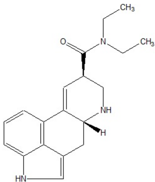
6-Norlysergic acid diethylamide
