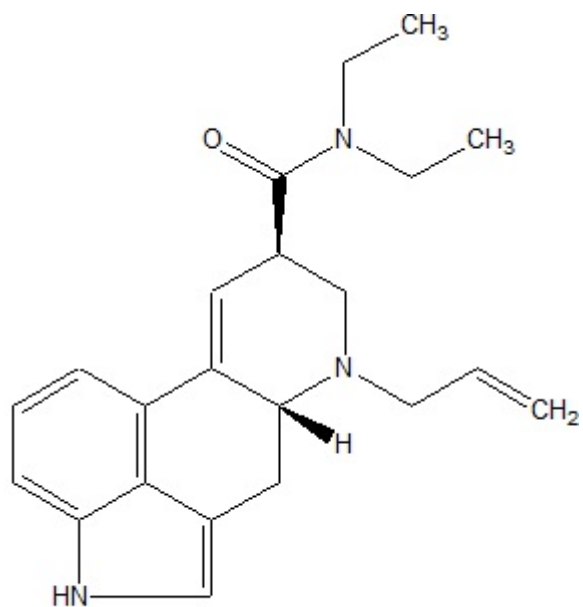
6-Nor-6-allyllysergic acid diethylamide
